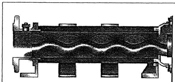
Figure 1. The progressive cavity pump works on the same principle as a screw pump. Rotor and stator are in continuous contact, therefore constantly wearing, as material is carried along through the pump. If the pump is shut off while pumping a dilatent slurry, material settles to the bottom of the cavity and begins to stiffen. When the pump is started, because the dilatent slurry is compressed by the rotor, the slurry stiffens and jams the rotor. Putting more horsepower on the shaft may tear the stator, resulting in a costly repair job. It is also possible for the connecting rod, knuckles, and seals to be damaged.
