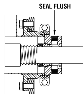
Drive end mechanical seal (Ceramic or Graphitar)
